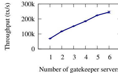
Figure 12: Throughput of get_node programs. Weaver scales linearly with the number of gatekeeper servers.
